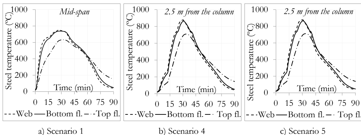
Figure 2.9: Temperature evolution in the secondary beam IPE 450
