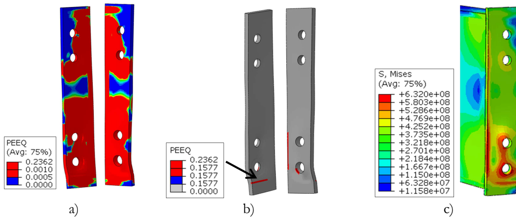
Figure 4.14: At the bolt failure: Equivalent plastic strain (PEEQ) in the end-plate corresponding to: a) the yielding ( f_y = 419 MPa; \varepsilon_y = 0.19\% ) and b) the ultimate stresses ( f_u = 539 MPa; \varepsilon_u = 17.3\% ); c) von Mises stresses
