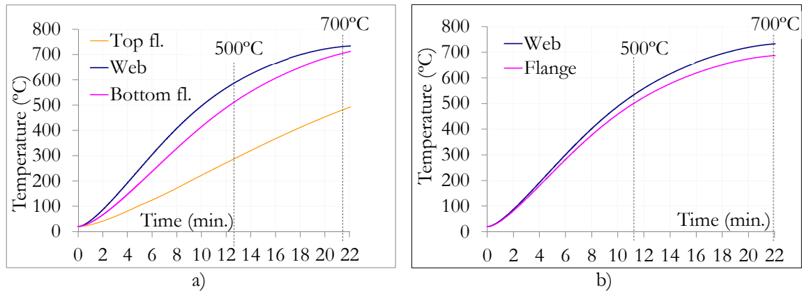
Figure D.3: ISO 834 fire up to 500^\circ\text{C} and 700^\circ\text{C} : a) Temperatures in the beam section, b) temperature in the column section
