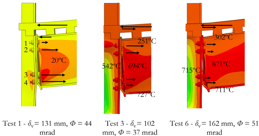
Figure 4.33: Deformation of the joints (scale x 2) and load distribution in the activated joint components
