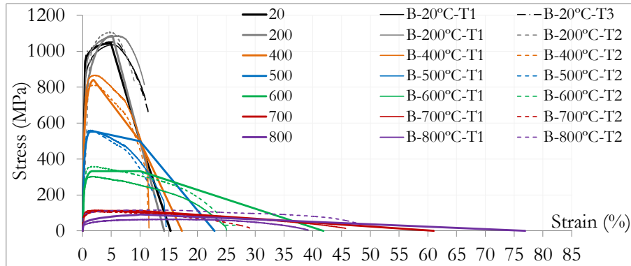
Figure A.20: Experimental and standardized stress-strain curves of bolts M30 grade 10.9 at 20^\circ\text{C} , 200^\circ\text{C} , 400^\circ\text{C} , 500^\circ\text{C} , 600^\circ\text{C} , 700^\circ\text{C} and 800^\circ\text{C}
