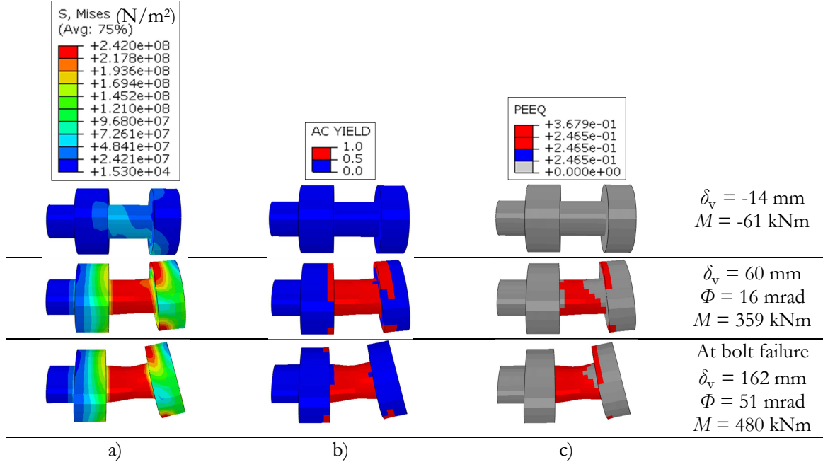
Figure 4.31: Evolution of the bottom bolt row deformation under sagging bending moment and 643°C (scale 1): a) von Mises stresses, b) Yielding, and c) Equivalent plastic strain PEEQ at failure ( \epsilon_{nom} \geq 30\% )
