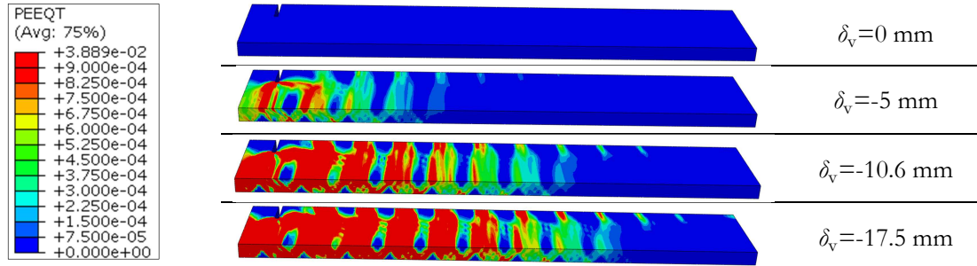
Figure 4.11: Evolution of the equivalent plastic strains in uniaxial tension (PEEQT) in the concrete slab during the application of the hogging bending moment ( f_{ct} \geq 2.9 MPa and \varepsilon_c \geq 0.01\% )
