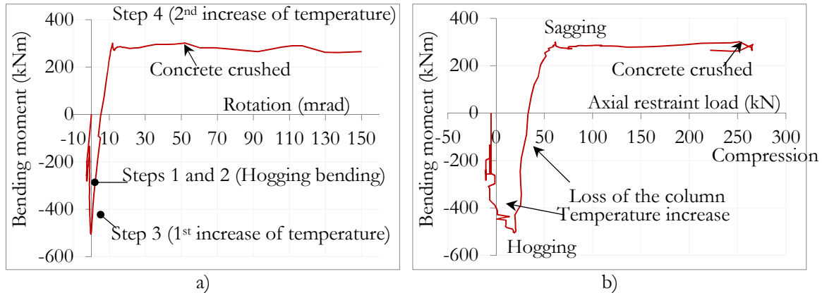
Figure 3.37: a) Joint bending moment versus rotation at the connection; b) Joint bending moment versus axial load restraint
