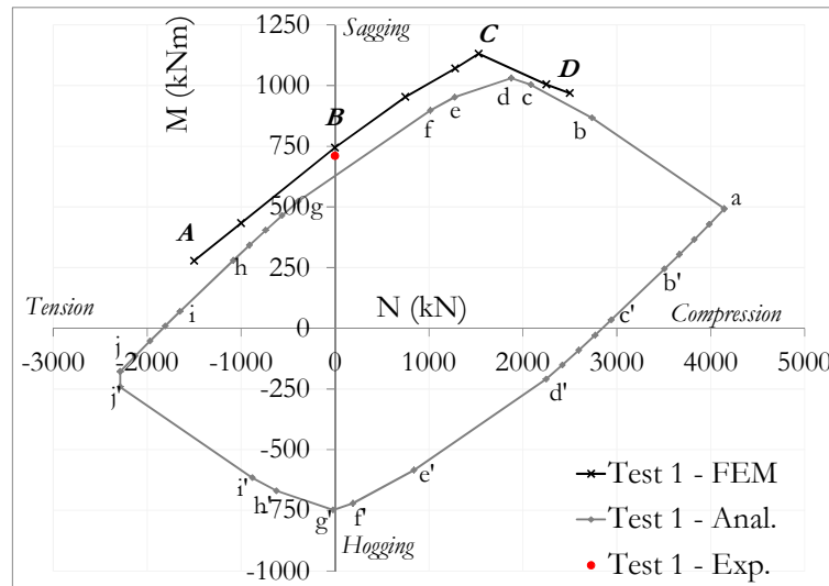
Figure 5.16: M-N curves at ambient temperature (test 1)
