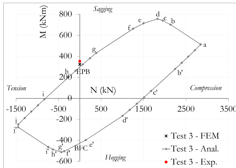
Figure 5.10: M-N curve at elevated temperatures (test 3)
