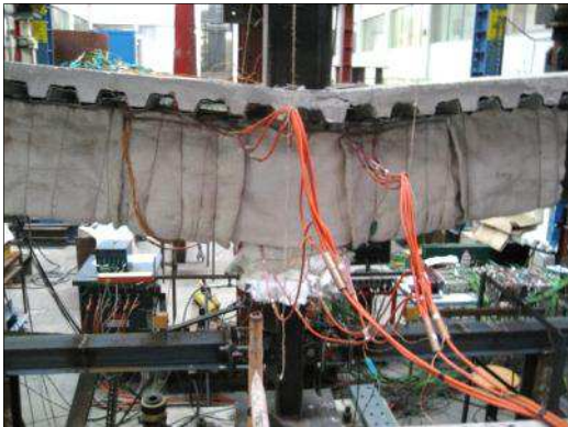
Figure B.18: Final deformation of the sub-frame (test 4 – 500°C and total axial restraint)
