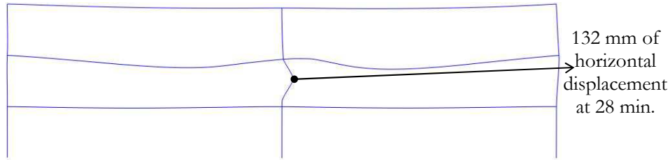
Figure 2.13: Frame deformation at 28 min of fire (scenario 4): column failure (scale 5)
