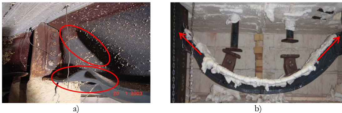
Figure 1.3: a) Local buckling of beam web in shear and beam flange in compression (Santiago, 2008); b) Catenary actions (Simões da Silva et al. , 2013)
