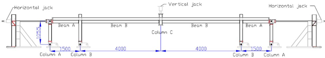
Figure 3.1: Sub-structure configuration tested at the University of Liège (Demonceau, 2008)
