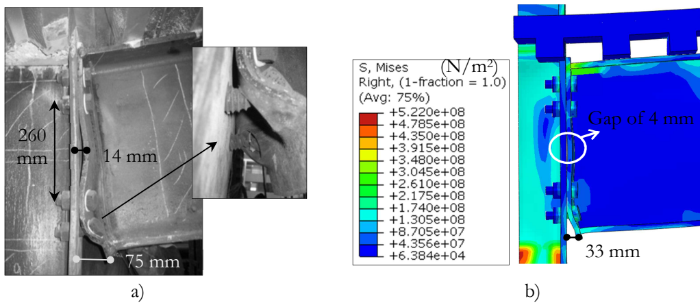
Figure 4.28: a) Deformation of the joint at the end of the experimental test ( \delta_v = 513 \text{ mm} ); b) FEM deformation of the joint when the bolt fails ( \delta_v = 163 \text{ mm} )
