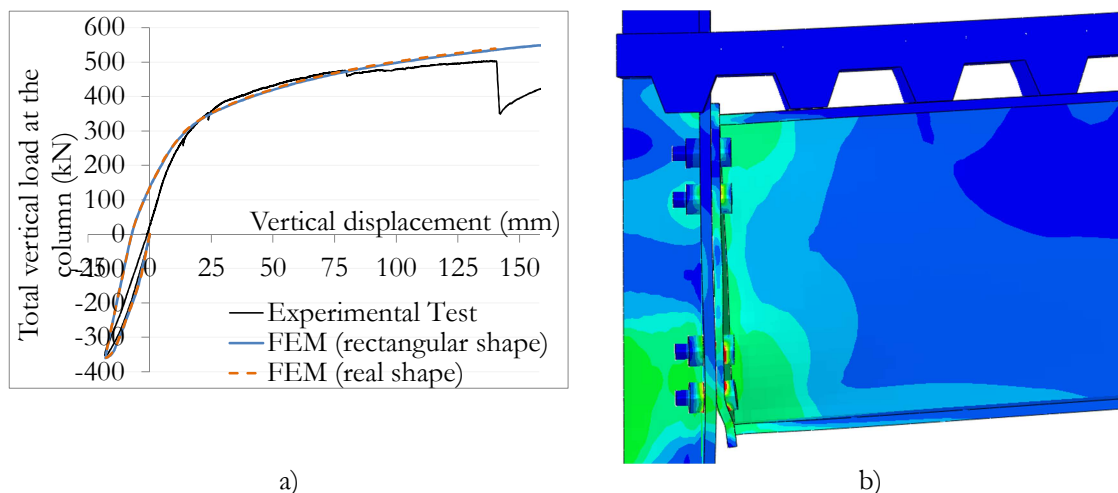
Figure D.6: Effect of the shape of the slab' ribs; a) Applied load - vertical displacement; b) FEM model with real shape of the ribs
