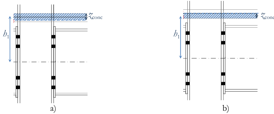
Figure 5.4: Variation of the thickness z_{\text{conc}} of the CSC component when the joint is subject to (a) M^+ and (b) M^-
