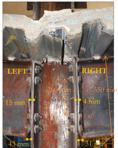
Figure B.21: Deformations of the joint (view from the front side / test 5 – 700°C and total axial restraint)
