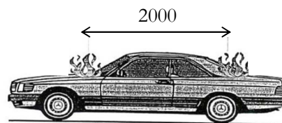
Figure 2.4: Front (F) and rear (R) fire plumes (ECCS, 1993)
